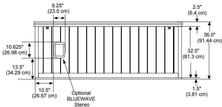
FRONT/BACK SIDE VIEW (Front view of stereo option shown) Tolerance: \pm 0.5" (1.27 cm)
