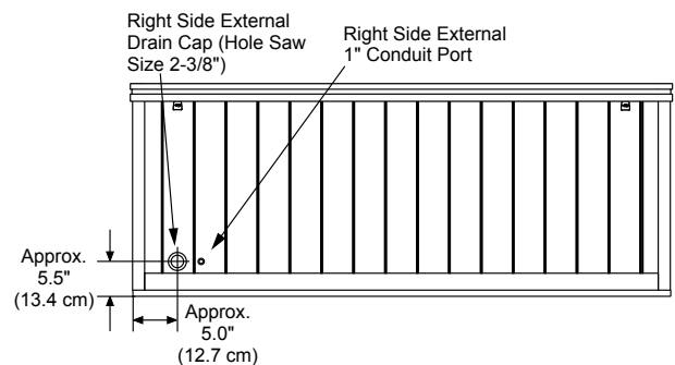
RIGHT SIDE VIEW Tolerance: \pm 0.5" (1.27 cm)
