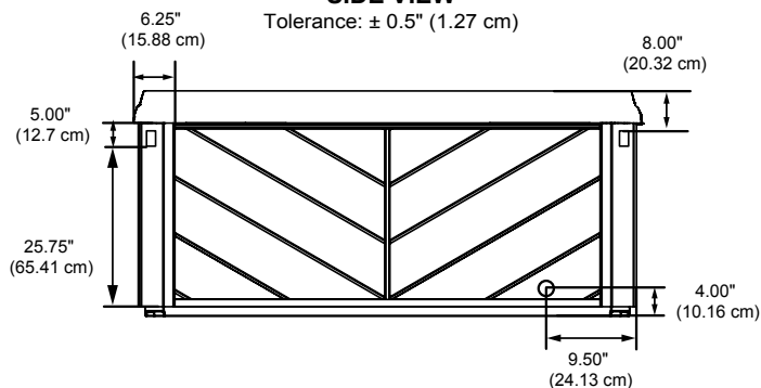
SIDE VIEW Tolerance: \pm 0.5" (1.27 cm)
